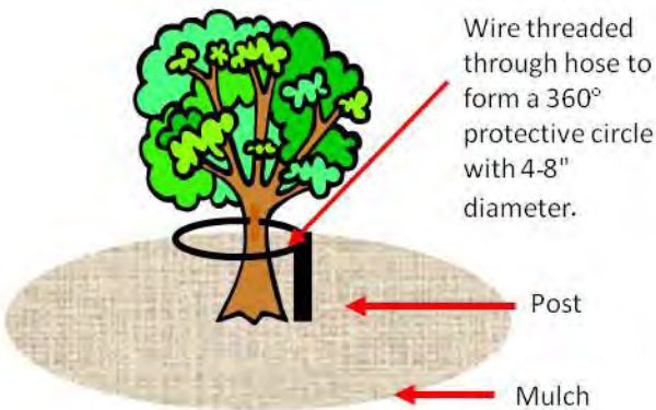
Figure 13: Staking With One Post
